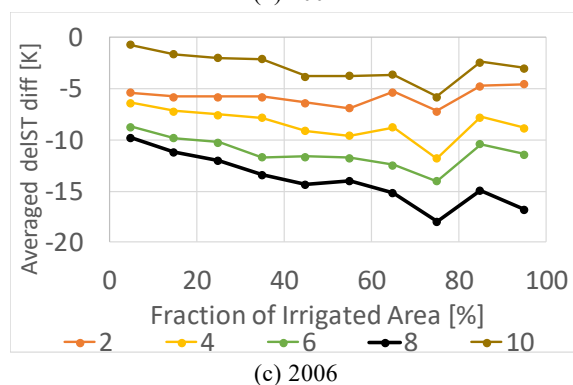
Fig.6 Monthly average of \Delta ST_{diff} in each irrigation fraction
