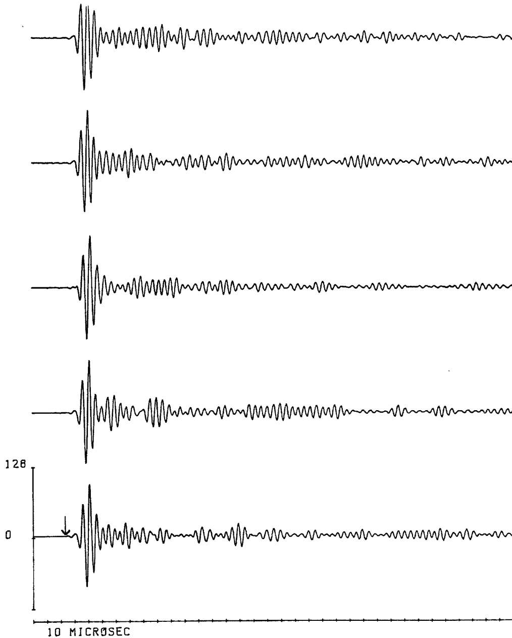
Fig. 4. Examples of seismograms produced by model experiments for the medium of Q=300 ( g=0.008 \text{ km}^{-1} and Q_{\text{scat}}=520 ): origin time being marked by an vertical arrow.
