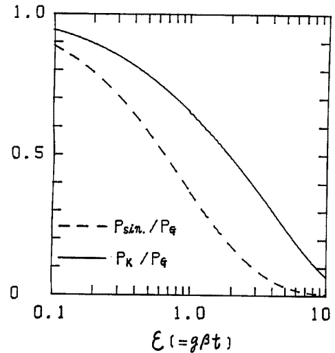
Fig. 1. Coda power ratio as a function of \epsilon : P_{sin} , power spectral density due to single scattering (by Aki and Chouet 2) ); P_K , that due to multiple scattering up to 3rd order (by Kopnischev 3) ); P_G , that due to multiple scattering up to 7th order (by Gao et al. 6) ); \epsilon , ratio of travel distance to mean free path l/g .
