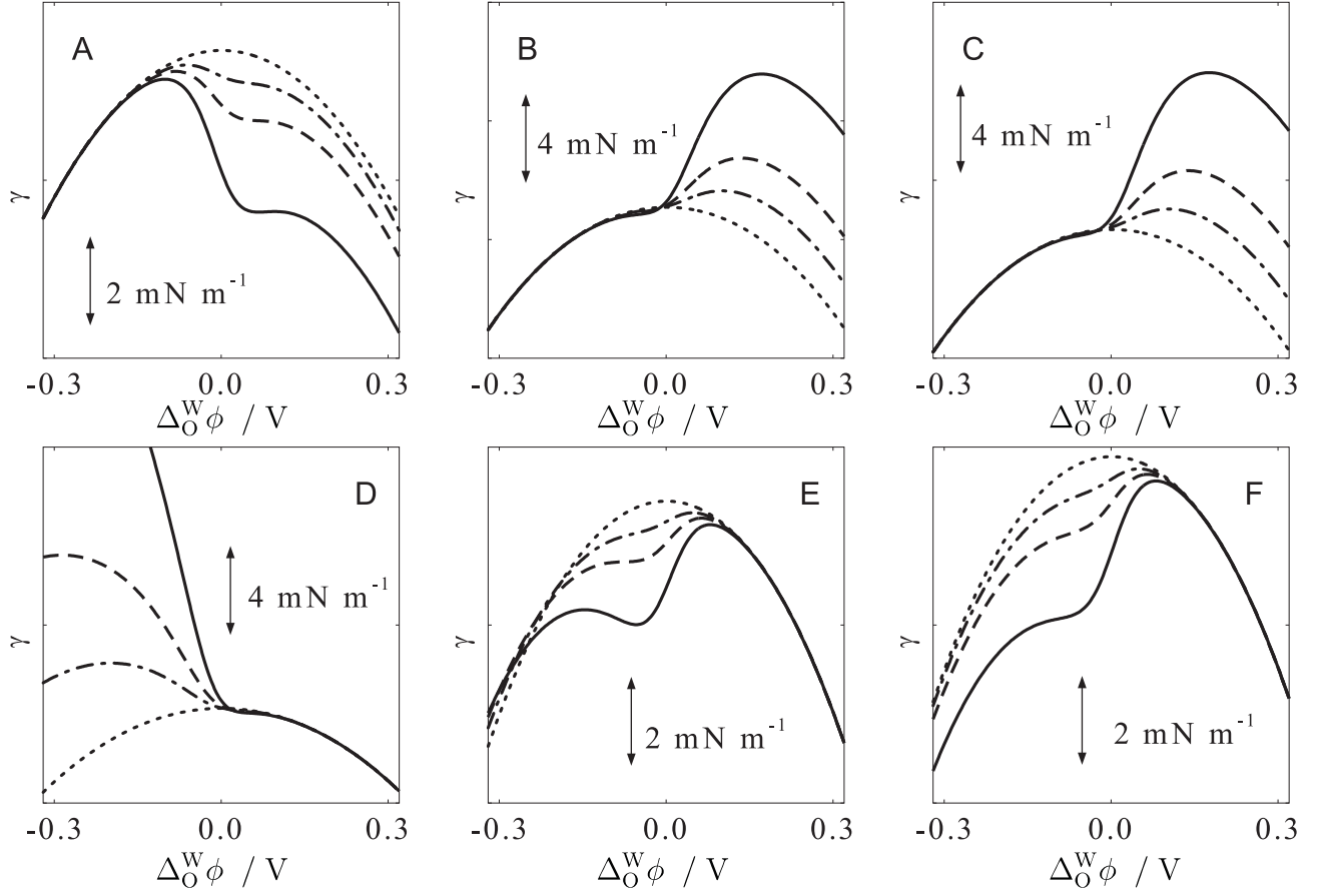
Figure 1.4: Effect of the position of the adsorbed surface-active ions and \beta parameters on the electrocapillary curves, when the adsorbed S exists at position I (A and D), II (B and E), and III (C and F) in Figure 1.1B. \beta is 0.3 (A, B, and C) and 0.9 (D, E, and F) and c_S is 0 (dotted lines), 50 (dash-dotted lines), 100 (broken lines), and 200 \text{mol m}^{-3} (solid lines).
