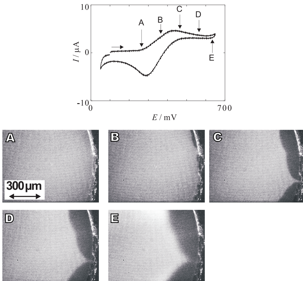
Figure 6.8: Voltammogram for the transfer of G4P across the DCE|W interface modified with 0.7 \mu\text{mol dm}^{-3} D3815 at v = 50 \text{ mV s}^{-1} , c_{\text{G4PCl}}^{\text{b,W}} = 1 \text{ mmol dm}^{-3} and simultaneously recorded fluorescent image of the interface. The alphabetic labels in the images correspond to that in the voltammogram.
