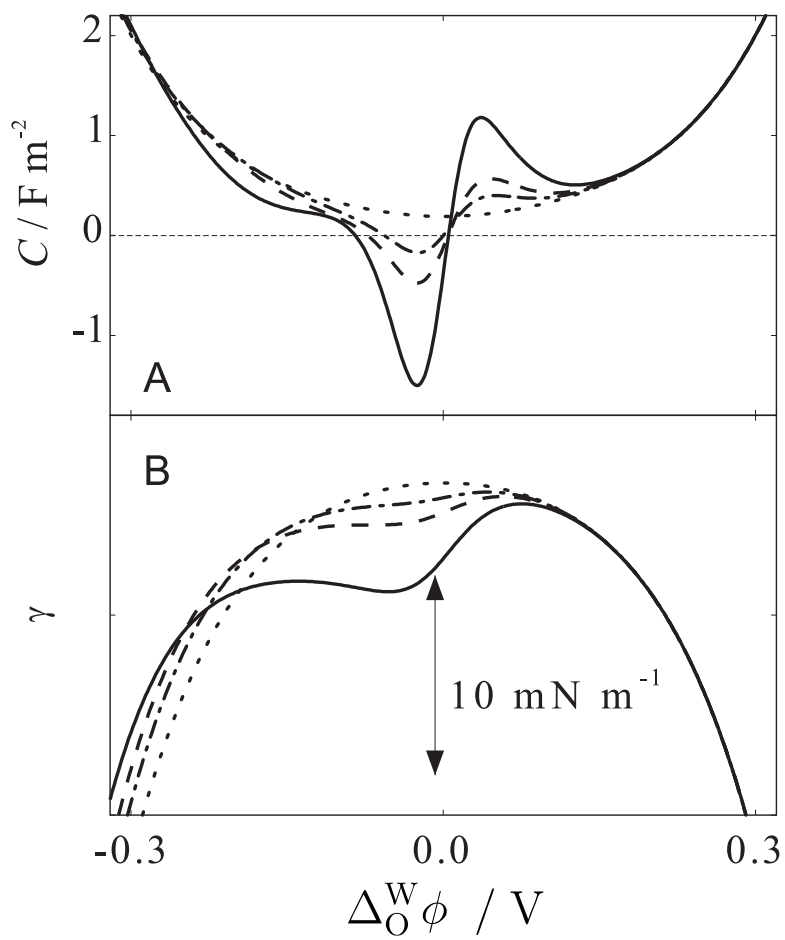
Figure 1.3: Potential-dependence of C (A) and \gamma (B), when c_S = 0 (dotted lines), 0.1 (dash-dotted lines), 0.2 (broken lines), and 0.5 mol m^{-3} (solid lines).
