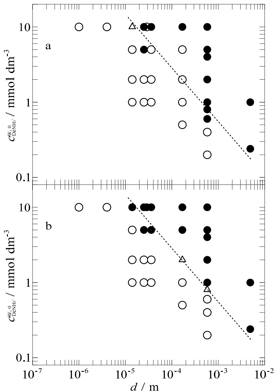
Figure 4.3: Effect of the inner diameter of the pipette orifice and the concentration of \text{DeNH}_3^+ on the appearance of the AIIC on voltammograms. v : 10 (a) and 200 \text{ mV s}^{-1} (b). Filled circle, open triangle, and open circle show the case when the AIIC was observed, occasionally observed, and not observed, respectively. Dashed lines show the demarcation between the filled circles and the open circles.
