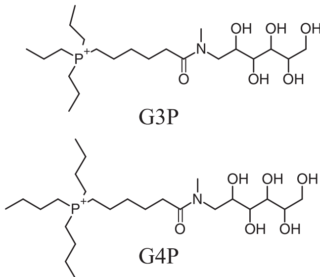
Figure 6.1: Structures of G3P and G4P.
