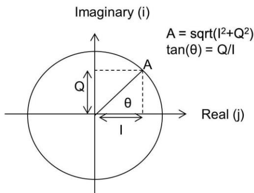
Figure 2.4 SAR data and statistic, composed by a real and imaginary part.
