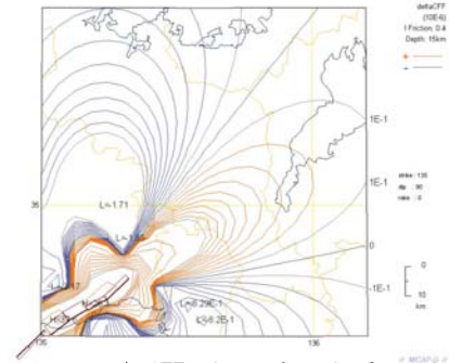
Fig. 9 \Delta CFF for the fault of strike= 135^\circ , dip= 90^\circ , rake= 180^\circ . Depth=15km.
