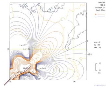
Fig. 7 \Delta CFF for the fault of strike= 45^\circ , dip= 90^\circ , rake= 180^\circ . Depth=15km.
