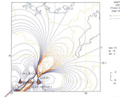
Fig. 11 \Delta CFF for the fault of strike= 115^\circ , dip= 90^\circ , rake= 180^\circ . Depth=3km.
