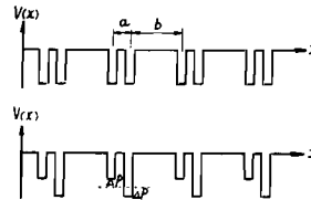
Fig. 14'. One-dimensional potential model used (after Seraphin).
