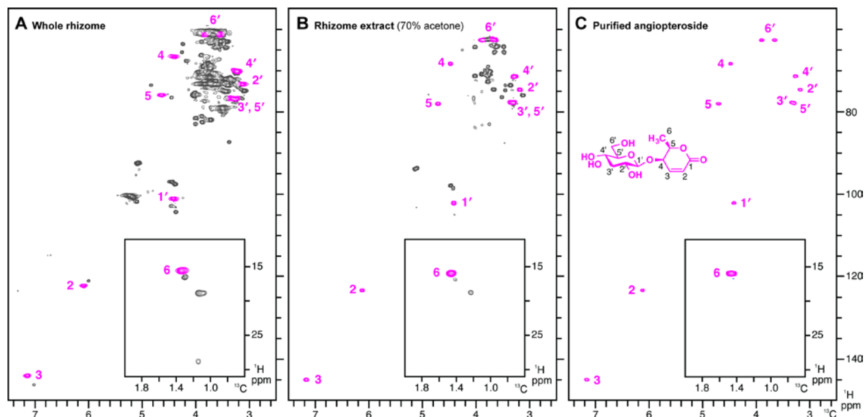
Figure 5. HSQC spectra of (A) a whole rhizome, (B) a rhizome extract (extract A 70 ), and (C) the purified angiopteriside (extract B)
