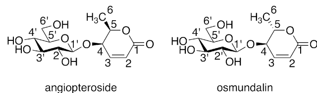
Figure 1. Chemical structures of angiopteroside and osmundalin
