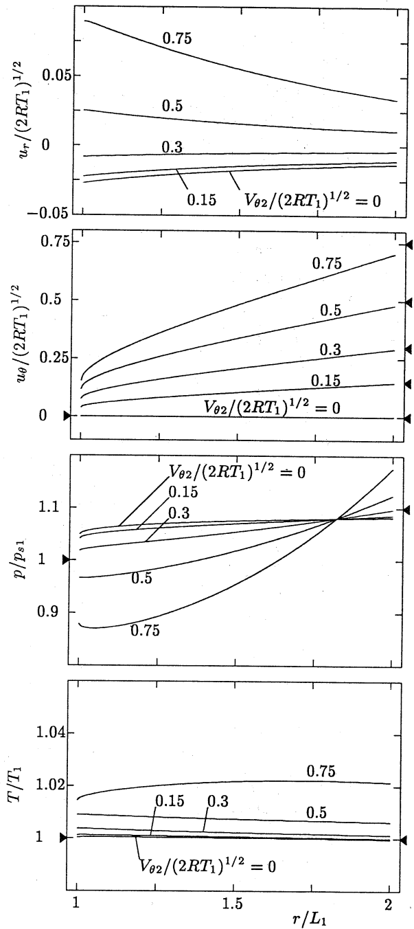
Fig. 6. The profiles of the flow velocity ( u_r , u_\theta ), pressure p , and temperature T of the gas for various circumferential velocities V_{\theta 2} of the outer cylinder when the inner cylinder is at rest II: ( \text{Kn} = 10 , p_{s2}/p_{s1} = 1.1 , T_2/T_1 = 1 , L_2/L_1 = 2 ). The symbol \blacktriangleright ( \blacktriangleleft ) indicates the position corresponding to V_{\theta 1} , p_{s1} , or T_1 ( V_{\theta 2} , p_{s2} , or T_2 ).
