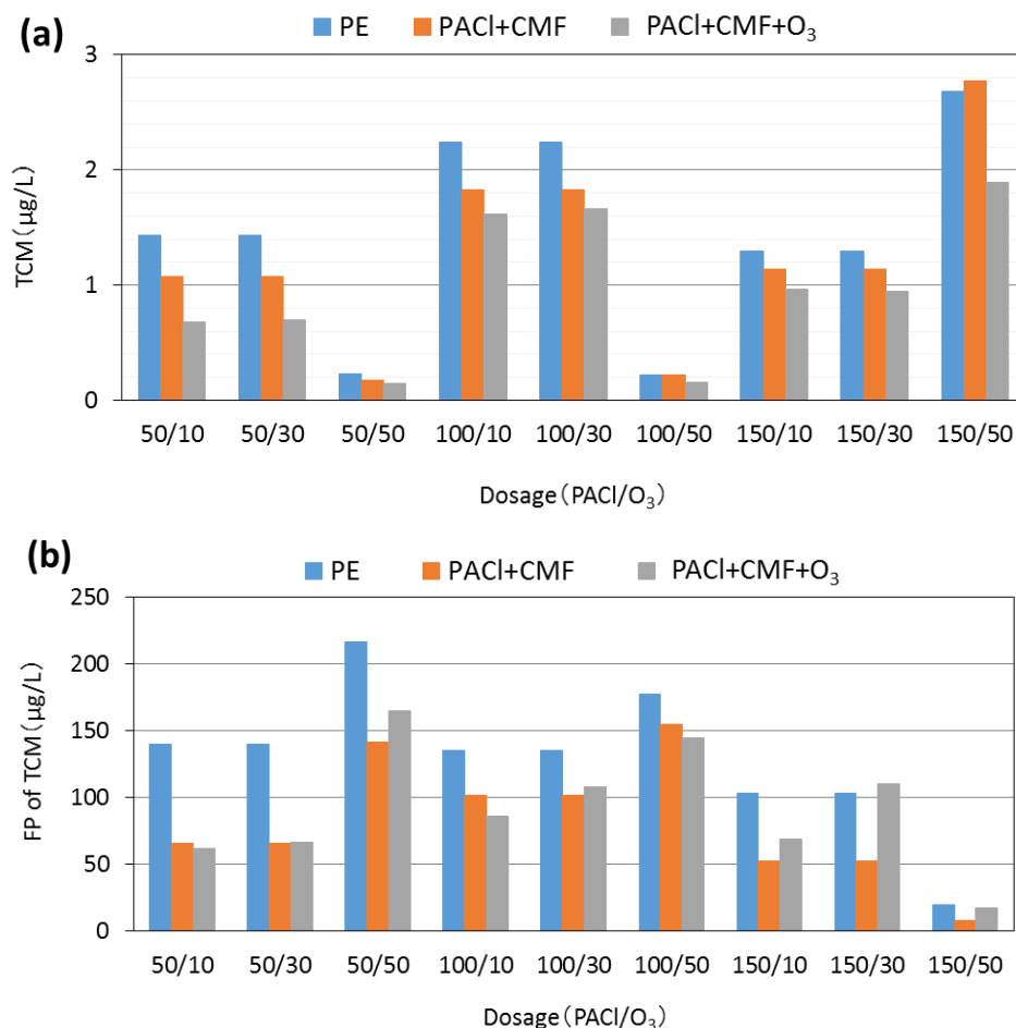
Figure 5.12 TCM concentration (a) and TCM FP (b) in PACI+CMF+O 3 for treating PE
