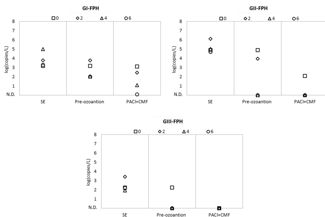
Figure 7.3 Concentrations of GI-FPH, GII-FPH and GIII-FPH in O 3 &CMF process for treating SE (Values on each figure represent O 3 dosage (mg-O 3 /L). PACI dosage was commonly 25 mg-PACI/L. N.D. means Not detected.)
