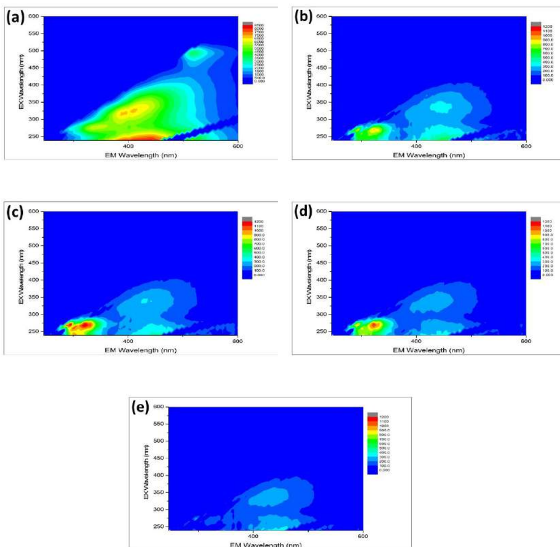
Figure 5.17 EEM spectra of (a) SE, (b) Pre-ozonated water, (c) BAC effluent, (d) Coagulated water and (e) CM permeate
