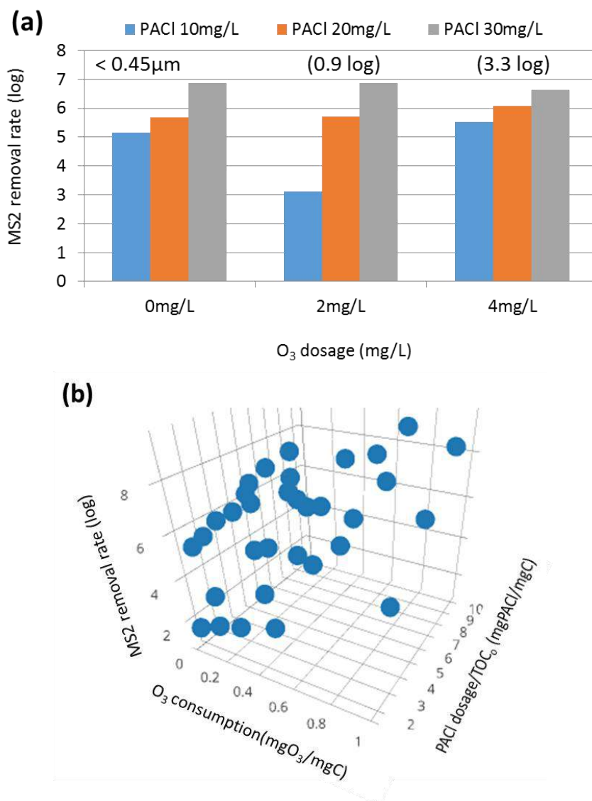
Figure 3.14 MS2 removal rate by ozonation and CS in SE represented by (a) bar plot and (b) 3D scatter plot (The parenthesis above bar plot represents MS2 removal rate by ozonation. MS2 removal rate by CS was calculated using MS2 concentration in liquid phase [<0.45 μm])
