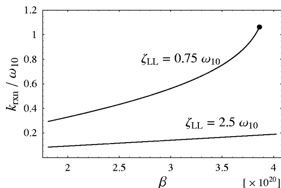
FIG. 16. The rate constant k_{\text{rxn}} calculated from Eq. (90) are plotted as a function of \beta for \zeta_{\text{LL}} = 0.75\omega_{10} and \zeta_{\text{LL}} = 2.5\omega_{10} within the high-temperature approximation and the nonadiabatic limit condition: \beta\hbar\gamma \ll 1 \ll \beta\hbar\omega_{\text{well}} . The other system-bath parameters are \zeta_{\text{SL}}' = 0.25\zeta_{\text{LL}}/\omega_{10} and \gamma = 6\omega_{10} . The closed circle denotes the crossover point \beta_c = 1/(k_B T_c) from the incoherent to the coherent phase. In the temperature region above T_c , the values of k_{\text{rxn}} decrease with increasing temperature. In the temperature below T_c , on the other hand, the rate constant k_{\text{rxn}} cannot be defined.
