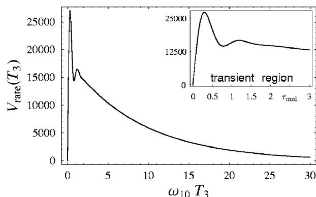
FIG. 14. The volume of the 2D signal in Fig. 13 is plotted as the function of the third delay time T_3 , where 1/\omega_{10} = 1.66 ps for \omega_{10} = 20 \text{cm}^{-1} . After the transient region T_3 < \tau_{\text{mol}} \sim 2.5/\omega_{10} , the volume decays exponentially with the reaction rate constant k_{\text{rxn}} : V_{\text{rate}}(T_3) \propto \exp(-k_{\text{rxn}} T_3) for T_3 > \tau_{\text{mol}} .
