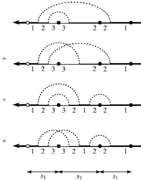
FIG. 3. Diagrammatic expression for the term of (J,K,L)=(3,2,1) in Eq. (23). Here, we have used the diagrammatic expression for \hat{G}_{13}[s] , \hat{G}_{32}[s] , and \hat{G}_{21}[s] in Fig. 2. The closed circle stands for the interaction with a pulse: \bullet = i/\hbar \cdot \mu(\hat{Q})^\times , while the open circle represents the dipole radiation to be observed: \circ = \mu(\hat{Q}) .
