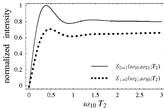
FIG. 7. Total intensity of the signals as the function of time T_2 given in Fig. 5, where 1/\omega_{10}=1.66 ps for \omega_{10}=20 cm ^{-1} . The solid line represents the total intensity S_{0 \rightarrow 1}(\omega_{30}, \omega_{21}; T_2) , which corresponds to the transition |0\rangle\langle 0| \rightarrow |1\rangle\langle 1| ; the dotted line represents the total intensity of S_{1 \rightarrow 0}(\omega_{21}, \omega_{30}; T_2) , which corresponds to |1\rangle\langle 1| \rightarrow |0\rangle\langle 0| . Since there are contributions from CP and CCP processes explained in Fig. 8, two lines do not agree.
