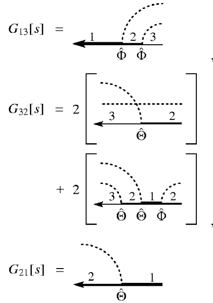
FIG. 2. Examples of the diagrammatic expression for G_{jk}[s] . A broken line denotes the one-photon excitation associated with \hat{\Theta} and \hat{\Phi} .
