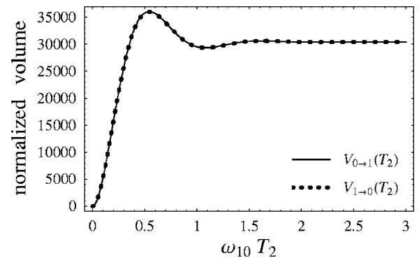
FIG. 9. The volume of the peak in Fig. 5 is plotted as the function of the time T_2 , where 1/\omega_{10}=1.66 ps for \omega_{10}=20 cm ^{-1} . The solid line is for the peak of S_{0 \rightarrow 1}(\Omega_1, \Omega_3; T_2) , which corresponds to the excitation |0\rangle\langle 0| \rightarrow |1\rangle\langle 1| , whereas the dotted line is for the peak of S_{1 \rightarrow 0}(\Omega_1, \Omega_3; T_2) , which corresponds to |1\rangle\langle 1| \rightarrow |0\rangle\langle 0| . By observing the volume of the cross peaks instead of the total intensity of the signals, we can separate the CT and CPP contributions from the net transition between the states.
