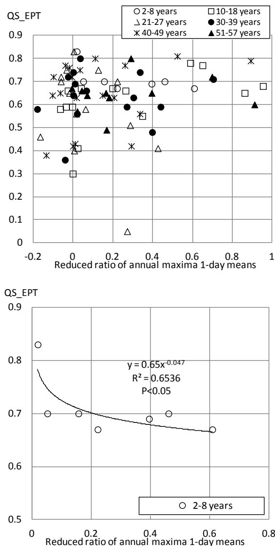
Fig. 1 Correlation between QS_EPT and reduced ratio of annual maxima 1-day means
