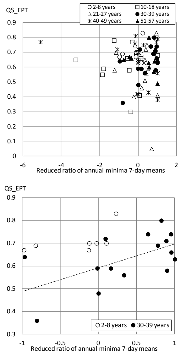
Fig. 2 Correlation between QS_EPT and reduced ratio of annual minima 7-day means
