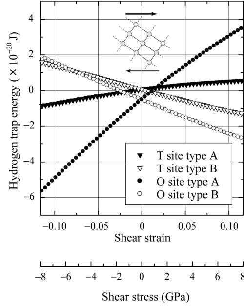
Fig. 8 Relationship between hydrogen-trap energy and applied simple shear: Shear stress calculated by \tau_{xy} = G\gamma is also shown in the horizontal axis. Here, G = 68.6 GPa is used.
