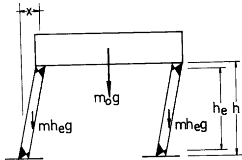
Fig. 13 Deformation Mode and Assumed Plastic Regions
