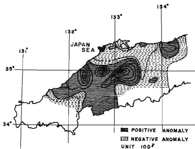
Fig. 3. Isoanomalic chart of the geomagnetic total intensity in the Chugoku district, 1960.
