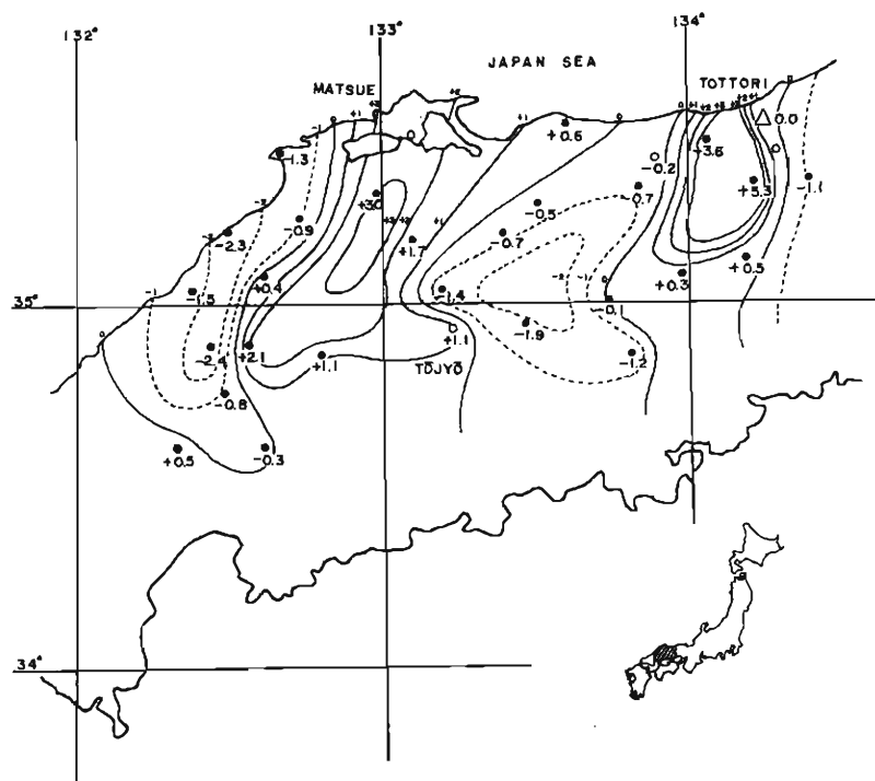
Fig. 2. The relative secular variation of the geomagnetic total intensity referring to the Tottori Micro-Earthquake Observatory, \Delta \dot{F}(\gamma/\text{year}) , in the Chugoku district from 1965 to 1971.
