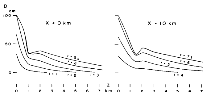
Figure 2. Dynamic displacements at short distances close to the fault surface, where X and Z are measured parallel and perpendicular to the fault from the point of rupture initiation, and t is the elapsed time. For other parameters, see text.
