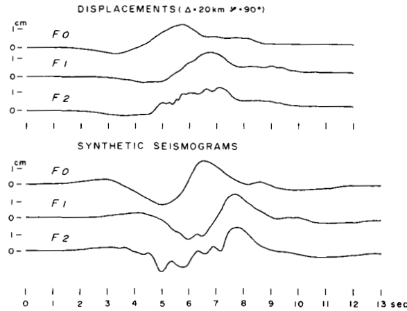
Figure 10. Near-field displacements (horizontal component parallel to the fault plane) from frictional faults, Cases F0, F1 and F2, and the corresponding synthetic seismograms at \Delta = 20 \text{ km} and \phi = 90^\circ .
