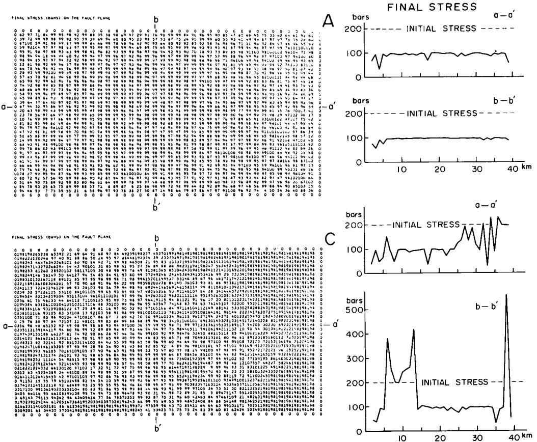
Figure 9. Distribution of the final stresses on the fault (left) and along the a-a' and b-b' axes (right) in Cases A and C. The initial stress level is indicated by broken lines.
