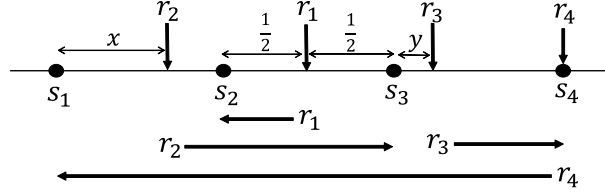
Fig. 5. Requests and ALG 's matching for Case 2-1 of Theorem 4.
