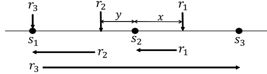
Fig. 2. Requests and ALG 's matching for Case 2-1 of Theorem 3.
