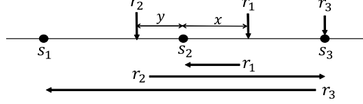
Fig. 3. Requests and ALG 's matching for Case 2-2 of Theorem 3.
