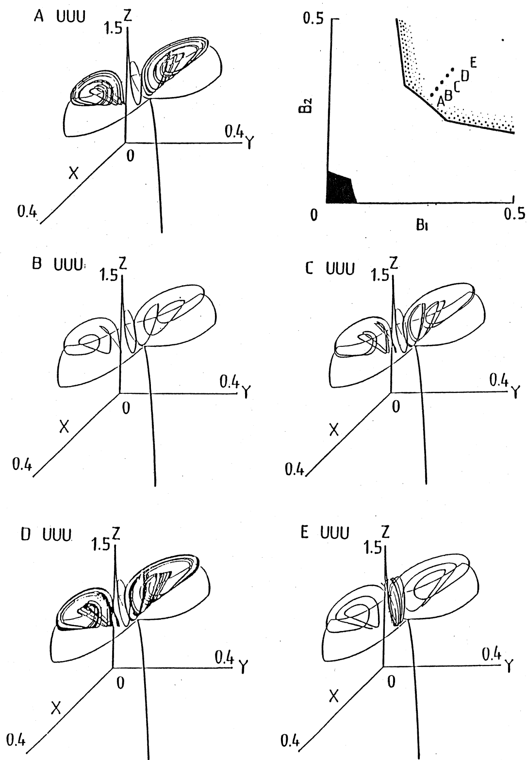
Fig.10 Bifurcation process
