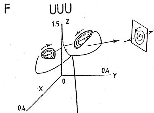
Fig.9 Typical nonlinear behavior in phase space
