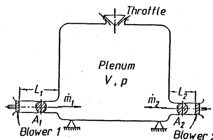
Fig.2 Parallel blower model
