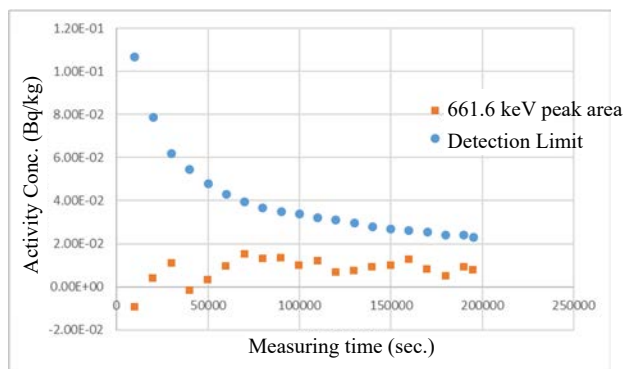
Fig. 2. Changes of activity concentration of 661.6 keV peak area and detection limit with respect to measurement time.
