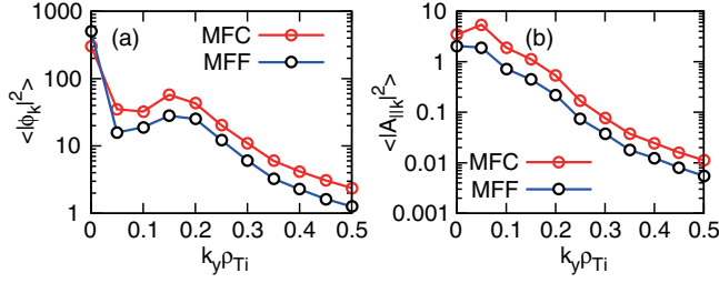
FIG. 3. Poloidal wave number spectra of (a) electrostatic potential \langle |\phi_k|^2 \rangle and (b) vector potential \langle |A_{||k}|^2 \rangle for MFC and MFF at \beta_i = 0.65\% .
