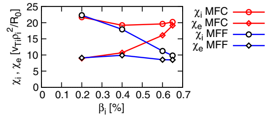
FIG. 2. Ion and electron energy diffusivity in the MFC and MFF as a function of \beta_i .
