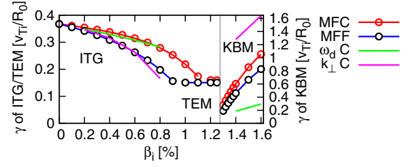
FIG. 1. Linear growth rate as a function of normalized ion pressure \beta_i in the magnetic field changed case (MFC, \alpha \neq 0 ) and in the magnetic field fixed case (MFF, \alpha = 0 ) at k_y \rho_{Ti} = 0.2 . The magnetic field changed only in \omega_d ( \omega_d C ) and only in k_\perp^2 ( k_\perp C ) cases are added.
