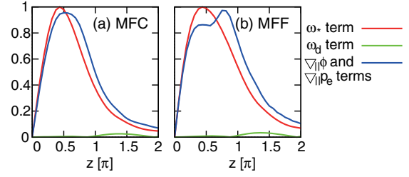
FIG. 5. Absolute values of the \omega_{*e} term, the \omega_{de} term, and the balance between the \nabla_{\parallel} \phi and \nabla_{\parallel} p_e terms in the electron parallel velocity equation for the linear eigenfunction at k_y \rho_{Ti} = 0.2 and \beta_i = 0.8\% for (a) the MFC and (b) the MFF.
