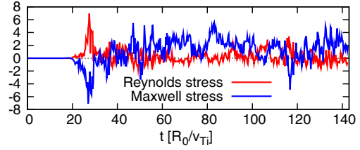
FIG. 4. Time history of zonal flow production by the Reynolds and Maxwell stresses for the MFC at \beta_i = 0.65\% .
