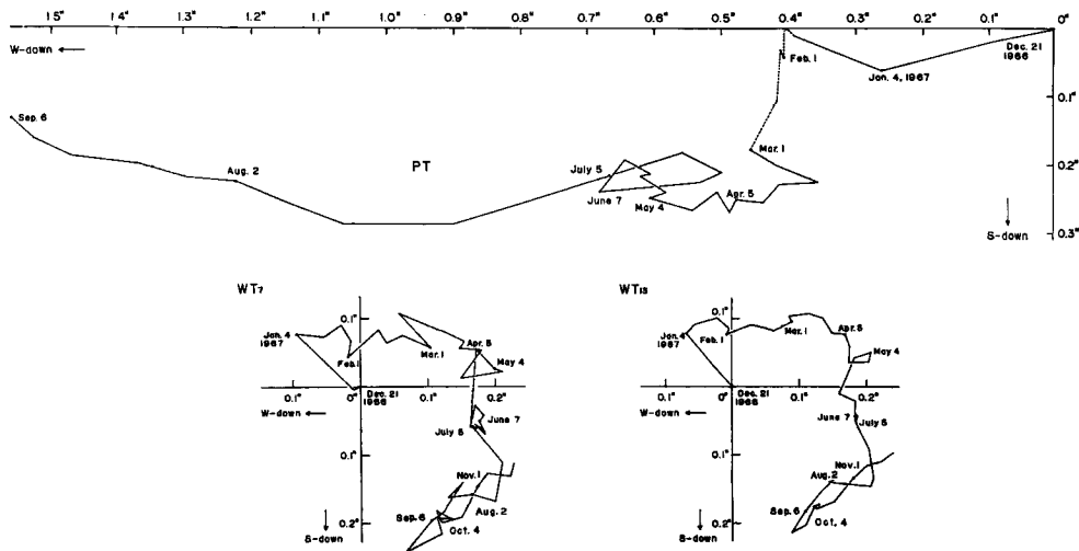
Fig. 6 Comparison of the vector of the ground tilt observed with the tiltmeters of horizontal pendulum type with that observed with the water-tube tiltmeters.
