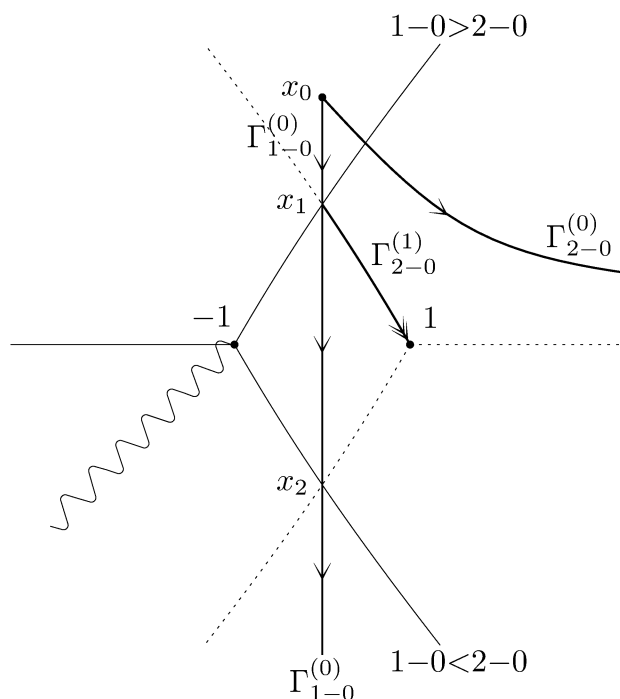
Figure 8. Exact steepest descent path passing through x_0 in Case (III).
