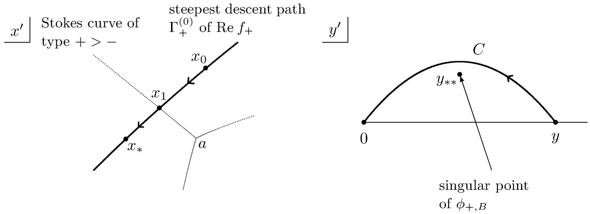
Figure 2. Integration path of (3.6) when y \geq \hat{y} .
