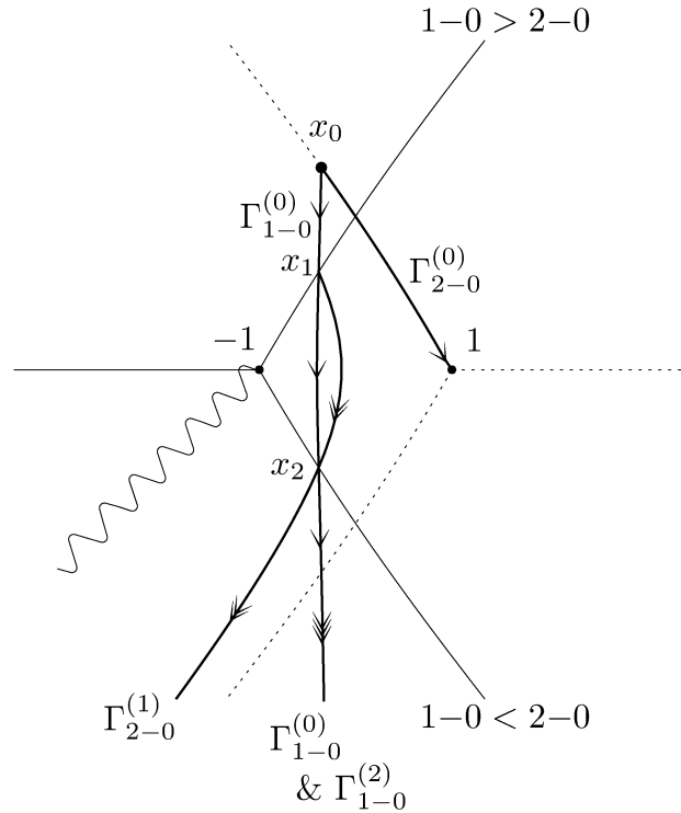
Figure 7. Exact steepest descent path passing through x_0 in Case (II).
