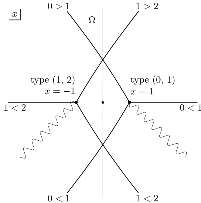
Figure 5. Stokes curves of the BNR equation (4.1).
