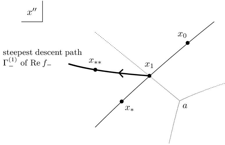
Figure 4. Integration path of (3.14).
