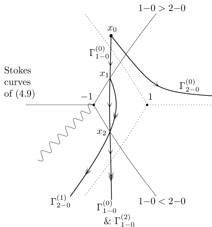
Figure 6. Exact steepest descent path passing through x_0 in Case (I).
