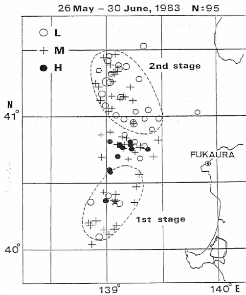
Fig.3 Epicenter distribution of the 1983 Nihonkai-Chubu earthquake (M7.7) from JMA data after Kuroiso et al. (1986). Symbols, L, M and H indicate frequencies of low, middle and high at the Abuyama Seismological Observatory. Earthquake ruptures preceded 1st stage to 2nd stage with a pause of about several seconds.
