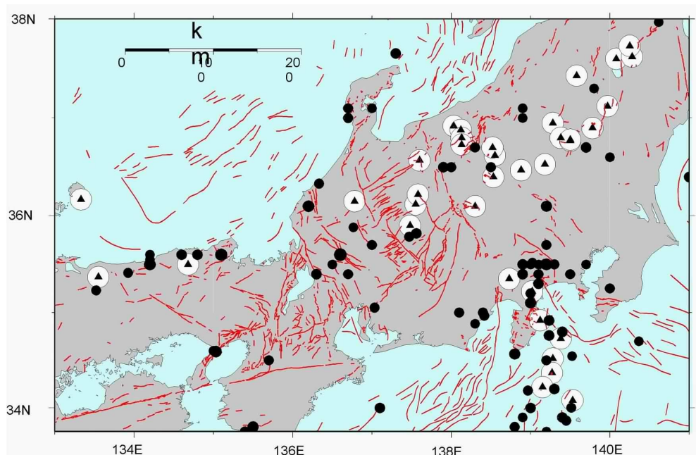
Fig.11 Distribution of the Quaternary volcanoes and large ( M \geq 6 ) earthquakes from 1885-2000. Circles show the area within 10km from each volcano.
