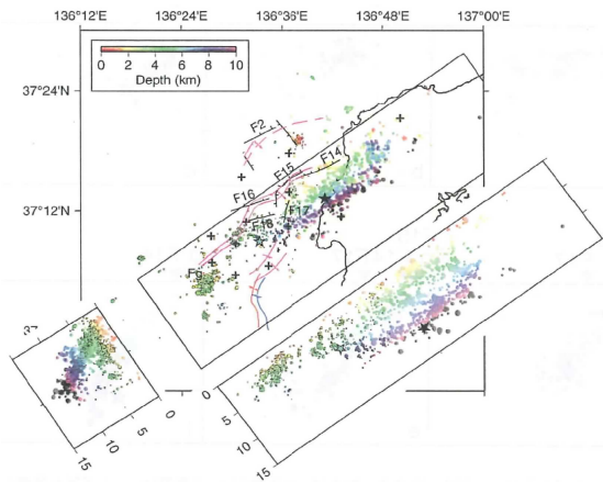
Fig.15 Distributions of epicenters and focal depths of aftershocks of the 2007 Noto earthquake M6.9 (Joint Observation of Aftershocks for the 2007 Noto Earthquake, 2007).
