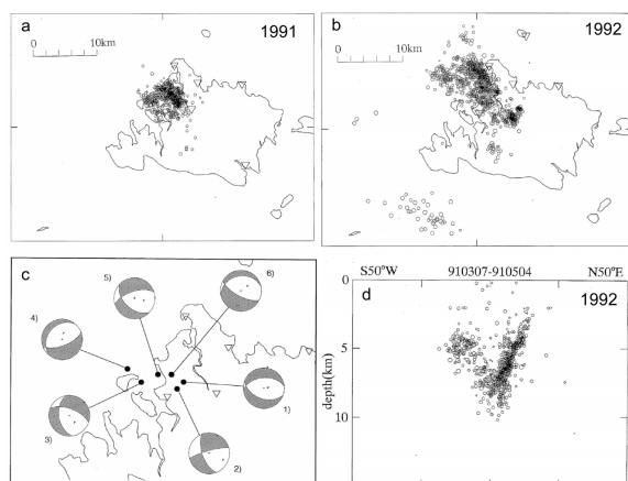
Fig. 6 Epicenter distributions of the Iriomote earthquake swarms in 1991 (a) and 1992 (b). Focal mechanisms of major events in 1992 with their epicenters (c) and focal depth section for 1992 events (d) is also shown (Shimizu et al., 1992).
