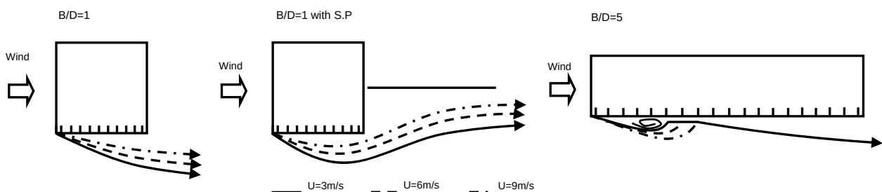
Fig. 6.5 Bluff body flow patterns around experimental models [Matsumoto, Shirato et al. 2006]
