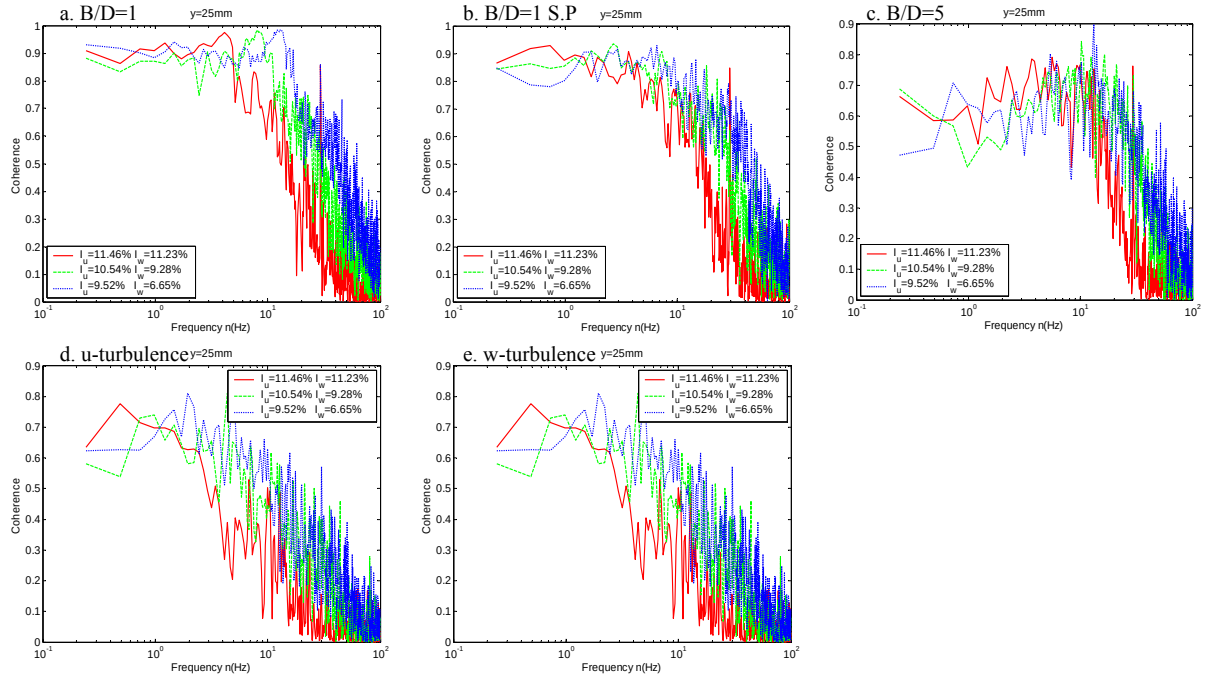
Fig. 5.9 Effect of turbulent flow conditions of pressure coherence: a. B/D=1, b. B/D=1 with S.P, c. B/D=5, d. u-turbulence, e. w-turbulence
