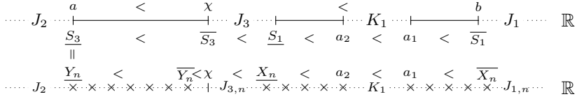
Figure 5.2. Top: An example support for possibilities (a) and (b). In words, S_1 is the union of two intervals, S_1 = [\underline{S_1}, a_2] \cup [a_1, \overline{S_1}] with \overline{S_1} > a_1 > a_2 > \underline{S_1} . Also, S_3 is a single interval, S_3 = [\underline{S_3}, \overline{S_3}] with \overline{S_3} > \underline{S_3} . Moreover, \underline{S_1} > \chi = \overline{S_3} , and so J_3 = (\chi, \underline{S_1}) and J_4 = \emptyset . Finally, K = K_1 = (a_2, a_1) . Bottom: Examples of the sets X_n and Y_n defined in (5.2). Elements of X_n and Y_n are denoted by \times .
