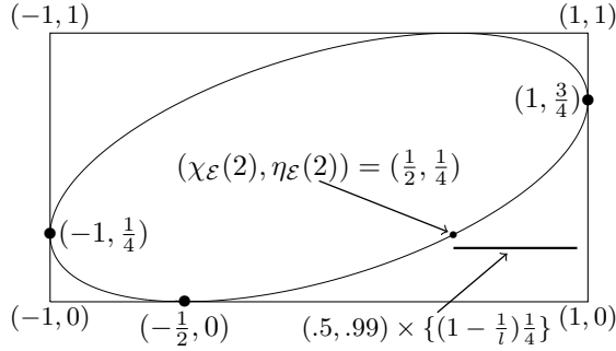
Figure 2.4. \mathcal{L} , \mathcal{E} and \mathcal{O} when \mu = \frac{1}{4}\delta_1 + \frac{3}{4}\delta_{-1} , and [.5, .99] \times \{(1 - \frac{1}{l})^{\frac{1}{4}}\} \subset \mathcal{O} . See Figure 2.3 for a more explicit description of \mathcal{L} , \mathcal{E} and \mathcal{O} in this case.
