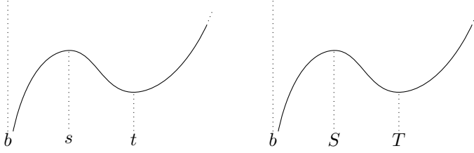
Figure 3.2. Left: The behaviour of y \mapsto f_{(\chi, \eta)}(y) for y \in (b, \infty) . Right: The behaviour of y \mapsto f_{(X, Y)}(y) for y \in (b, \infty) .
