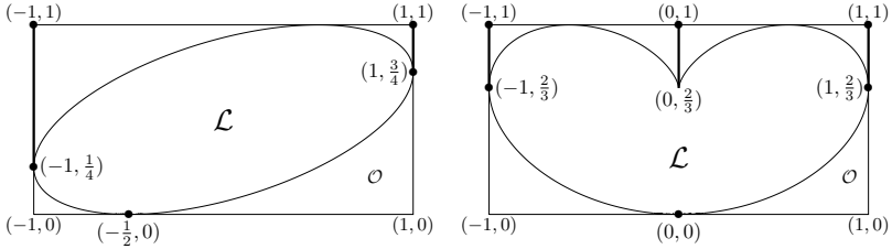
Figure 2.3. Left: \mu = \frac{1}{4}\delta_1 + \frac{3}{4}\delta_{-1} . \mathcal{E} is composed of all points on \partial\mathcal{L} except the lower tangent point (\int_a^b x\mu[dx], 0) = (-\frac{1}{2}, 0) . Right: \mu = \frac{1}{3}\delta_1 + \frac{1}{3}\delta_0 + \frac{1}{3}\delta_{-1} . \mathcal{E} is composed of all points on \partial\mathcal{L} except the lower tangent point (\int_a^b x\mu[dx], 0) = (0, 0) . In both cases \lim_{t \rightarrow \pm\infty} (\chi_{\mathcal{E}}(t), \eta_{\mathcal{E}}(t)) equals the lower tangent point, and parameter increases in the clockwise direction.
