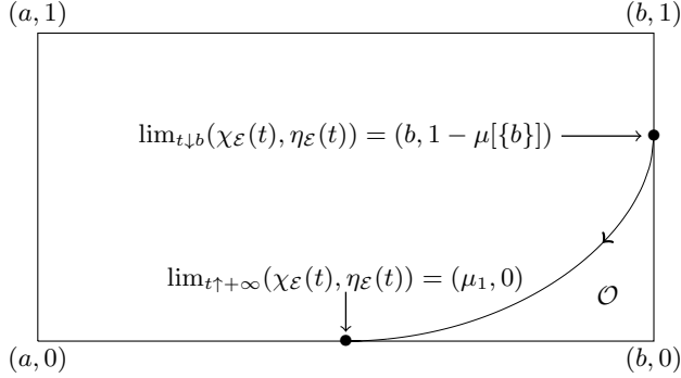
Figure 2.2. (\chi_\varepsilon(\cdot), \eta_\varepsilon(\cdot)) : (b, +\infty) \rightarrow \mathcal{E} when \mu[\{b\}] > 0 . The arrow represents the direction of the increasing parameter, and \mu_1 := \int_a^b x \mu[dx] .
