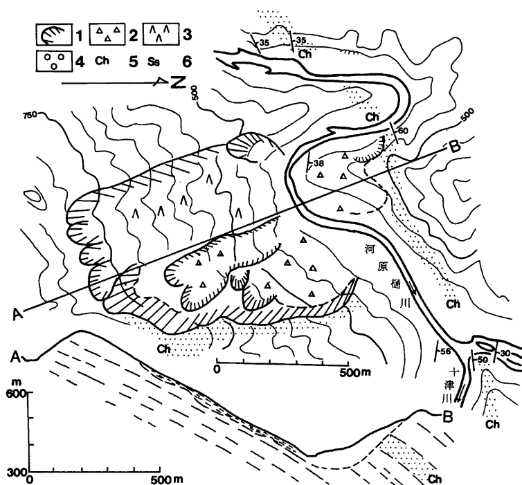
Fig. 7 Topography, geology and schematic cross-section of the landslide at Hinose-yama facing the Kitarabiki river, Nara Prefecture.
