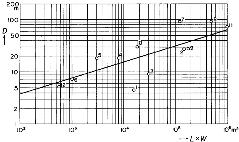
Fig. 5 Relationship of the landslide area in the abscissa to its depth in the ordinate. Area and depth are represented in the unit of \text{m}^2 and m, respectively.
