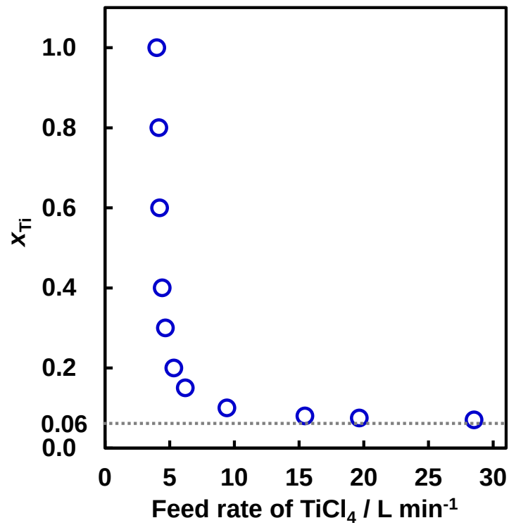
Figure 8 Relationship between x_{Ti} and the feed rate of TiCl_4 determined by the heat balance consideration in the reduction step. Suppose the feed rate of TiCl_4 in the Kroll process is 4\ L\ min^{-1} [8,9].
