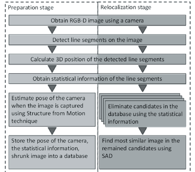
Fig. 1. Configuration of the proposed relocalization method.
