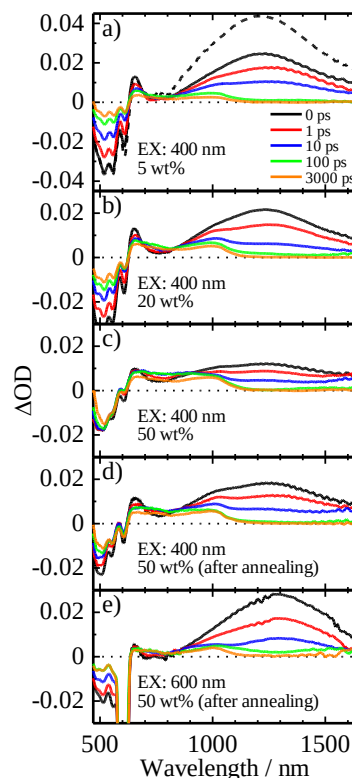
Fig. 6.8 Transient absorption spectra of RR-P3HT pristine (broken line in the panel a) and RR-P3HT/PCBM blend (solid lines) films measured at 0 (black), 1 (red), 10, (blue), 100 (light green), and 3000 (orange) ps after the laser excitation. The excitation wavelengths were a–d) 400 nm ( \sim 15 \mu\text{J cm}^{-2} ) and e) 600 nm ( \sim 10 \mu\text{J cm}^{-2} ). The PCBM concentrations were a) 5, b) 20, and c–e) 50 wt%. The spectra in the panels d and e were measured after thermal annealing at 140 °C for 30 min. The \Delta\text{OD} was corrected for variations in the absorption at the excitation wavelength. Reprinted with the permission from ref. [27]. Copyright 2010 American Chemical Society.
