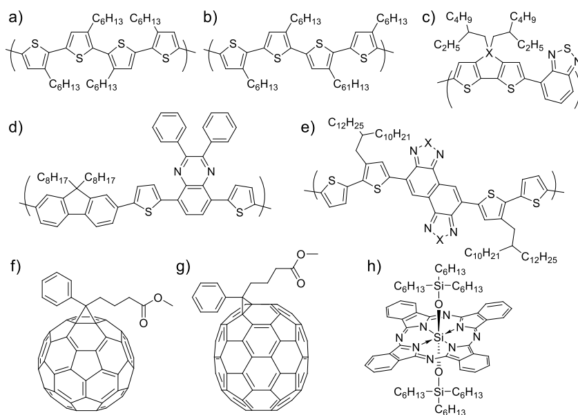
Fig. 6.5 Chemical structures of photovoltaic materials studied in this chapter: a) RRa-P3HT, b) RR-P3HT, c) PCPDTBT (X = C), PSBTBT (X = Si), d) NP-7, e) PNTz4T (X = S), PNOz4T (X = O), f) PCBM, g) PC 71 BM, and h) SiPc6.
