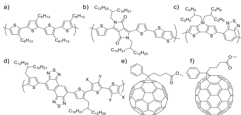
Fig. 6.15 Chemical structures of photovoltaic materials studied in this chapter: a) RR-P3HT, b) DT-PDPP2T-TT, c) PSBTBT, d) PNTz4T (X = Y = H), PNTz4TF2 (X = H, Y = F), PNTz4TF4 (X = Y = F), e) PCBM, and f) PC 71 BM.
