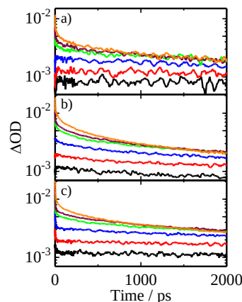
Fig. 6.9 Transient absorption signals measured at a) 700, b) 850, and c) 1000 nm of RR-P3HT/PCBM (50 wt%) blend films excited at 400 nm with a fluence of 6, 12, 24, 48, 72, and 120 \mu\text{J cm}^{-2} from top to bottom in each panel. Reprinted with the permission from ref. [27]. Copyright 2010 American Chemical Society.
