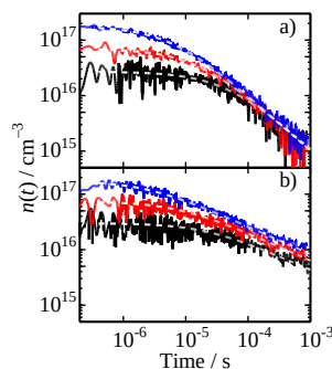
Fig. 6.17 Charge density decays of RR-P3HT/PCBM blend films excited at 400 nm with a fluence of 0.8 (blue lines), 1.8 (red lines), and 4.7 \mu\text{J cm}^{-2} (black lines). The spectra were measured at a) 700 nm and b) 1000 nm. The broken lines represent fitting curves with an empirical equation: n(t) = n(0)/(1 + at)^\alpha . Reprinted with the permission from ref. [44]. Copyright 2010 American Chemical Society.
