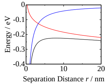
Fig. 6.20 The Coulomb potential energy \Delta H (blue line), the entropy contribution -T\Delta S (red line), and the Gibbs free energy \Delta G (black line) for an electron-hole pair at a separation distance r . The dielectric constant is assumed to be 3.5. The entropy term is calculated for 3D aggregates with a lattice constant of 1 nm.
