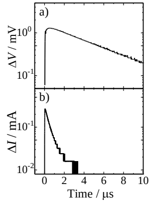
Fig. 6.19 a) TPV and b) TPC decays of RR-P3HT/PCBM solar cells under 1 sun illumination. Adapted with the permission from ref. [45]. Copyright 2016 The Society of Photopolymer Science and Technology.
