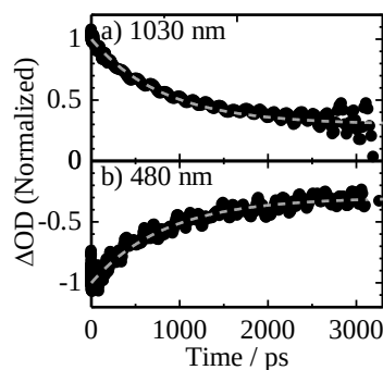
Fig. 6.7 Transient absorption decays of RRa-P3HT/PCBM blend films excited at 400 nm with a fluence of \sim 12 \mu\text{J cm}^{-2} , which were measured at a) 1030 nm and b) 480 nm. The decays were fitted with an exponential function and a constant: \Delta\text{OD}(t) = A_D \exp(-t/\tau_D) + B . The broken lines represent the best-fitting curves. Reprinted with the permission from ref. [27]. Copyright 2010 American Chemical Society.
