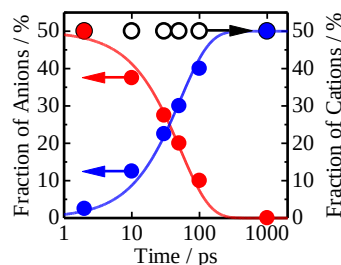
Fig. 6.14 The fraction of SiPc6 anions (red circles), PCBM anions (blue circles), and P3HT polarons (open circles) in RR-P3HT/PCBM/SiPc6 ternary blend films after the laser excitation of SiPc6 at 680 nm with a fluence of 7 \mu\text{J cm}^{-2} . Adapted with the permission from ref. [13]. Copyright 2010 American Chemical Society.
