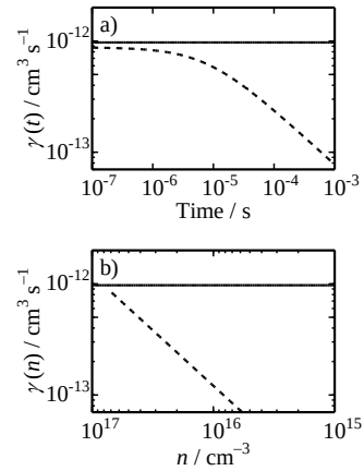
Fig. 6.18 Log-log plots of the bimolecular recombination rate as a function of a) time t (Eq. (6.5)) and b) carrier density n (Eq. (6.6)). The solid and broken lines represent the bimolecular recombination rate for the charge carriers observed at 700 and 1000 nm, respectively. Adapted with the permission from ref. [44]. Copyright 2010 American Chemical Society.
