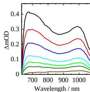
Fig. 6.16 Transient absorption spectra of RR-P3HT/PCBM blend films excited at 400 nm with a fluence of 30 \mu\text{J cm}^{-2} . The spectra were measured at 0.5 (black), 1 (red), 2 (blue), 5, (light blue), 10 (light green), 20 (green), and 100 \mu\text{s} (brown). Adapted with the permission from ref. [44]. Copyright 2010 American Chemical Society.
