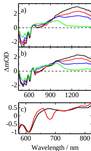
Fig. 6.12 Transient absorption spectra of a) RR-P3HT/PCBM and b) RR-P3HT/PCBM/SiPc6 blend films measured at 0 (black), 1 (red), 10, (blue), and 100 (light green) ps after the laser excitation. The excitation wavelength and intensity were 400 nm and 6 \mu\text{J cm}^{-2} , respectively. c) Transient absorption spectra of RR-P3HT/PCBM (black line) and RR-P3HT/PCBM/SiPc6 (red line) blend films measured at 10 ps. Adapted with the permission from ref. [13]. Copyright 2010 American Chemical Society.
