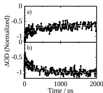
Fig. 6.10 Transient absorption signals of RR-P3HT/PCBM (50 wt%) blend films excited at 400 nm ( \sim 12 \mu\text{J cm}^{-2} ), measured at a) 480 and b) 610 nm, which were fitted by \Delta\text{OD}(t) = A_R[1 - \exp(-t/\tau_R)] + B and \Delta\text{OD}(t) = A_D \exp(-t/\tau_D) + B , respectively. The broken lines represent the best-fitting curves. Adapted with the permission from ref. [27]. Copyright 2010 American Chemical Society.
