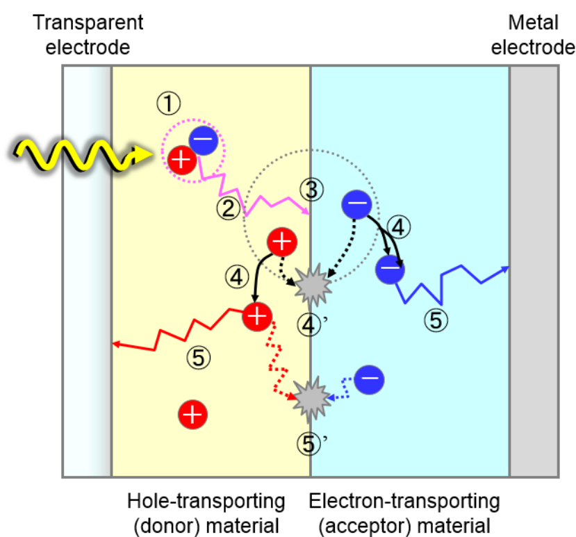
Fig. 6.1 Elementary processes of photovoltaic conversion in polymer solar cells with a bilayered device structure based on donor (light yellow part) and acceptor (light blue part) materials. (1) exciton generation upon photon absorption by the donor material, (2) exciton diffusion into a donor/acceptor interface, (3) charge transfer from the exciton arriving at the interface, (4) charge dissociation into free charge carriers, (4') geminate (monomolecular) recombination of an electron-hole pair at the charge transfer state, (5) charge collection of free charge carriers to each electrode, and (5') non-geminate (bimolecular) recombination of free charge carriers.
