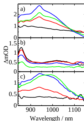
Fig. 6.13 Transient absorption spectra of a) RR-P3HT/SiPc6, b) PCBM/SiPc6 binary, and c) RR-P3HT/PCBM/SiPc6 ternary blend films measured at 0 (black), 1 (red), 10, (blue), and 200 (light green) ps after the laser excitation. The excitation wavelength and intensity were 680 nm and 7 \mu\text{J cm}^{-2} , respectively. Adapted with the permission from ref. [13]. Copyright 2010 American Chemical Society.
