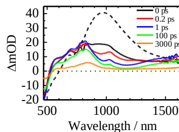
Fig. 6.6 Transient absorption spectra of RRa-P3HT pristine (broken line) and RRa-P3HT/PCBM blend (solid lines) films measured at 0 (black), 0.2 (red), 1 (blue), 100 (light green), and 3000 (orange) ps after the laser excitation. The excitation wavelength was 400 nm ( \sim 30 \mu\text{J cm}^{-2} ). The \Delta\text{OD} was corrected for variations in the absorption at the excitation wavelength. Adapted with the permission from ref. [27]. Copyright 2010 American Chemical Society.
