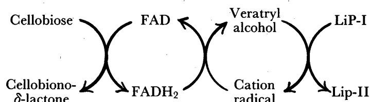
Fig. 1. Mechanism for the redox interaction between LiP and CBQ (FAD/FADH 2 ) proposed by Samejima and Eriksson.
