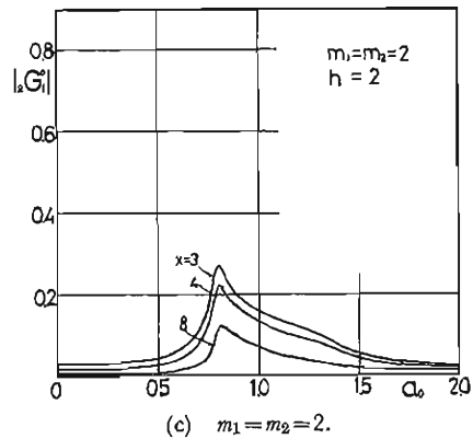
Fig. 10. Displacement amplitude characteristics of the passive mass of two-mass system to force excitation, h=2 .
