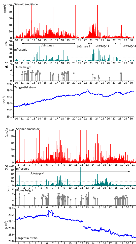
Fig.3 Seismicity, eruptive activity and ground deformation during the period from August 10 to 30, 2017 (Top) and September 1 to 21 (Bottom).
