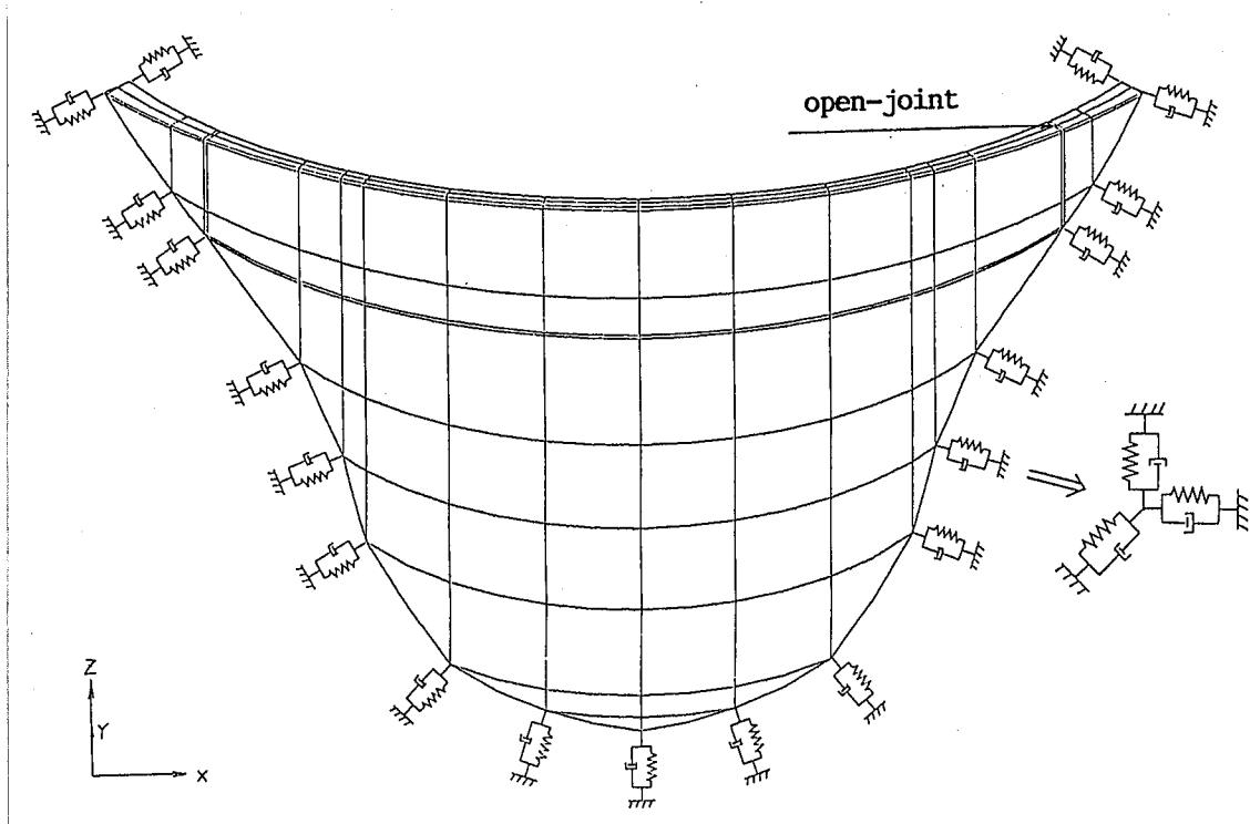
Figure 2.2.18 Finite element model with far-field impedance along the dam-foundation interface
