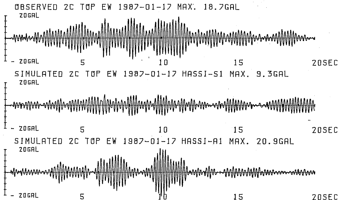
Figure 2.3.11(d) Comparison of acceleration time histories (EW components) between the observed and simulated: The upper is the observed motion of the roof top of the model, the middle the simulated motion by using the S1 motion, and the lower that by using the A1 motion ( r=1.8 t/cu.m, V_s=275 m/s, h=0.5\% ).
