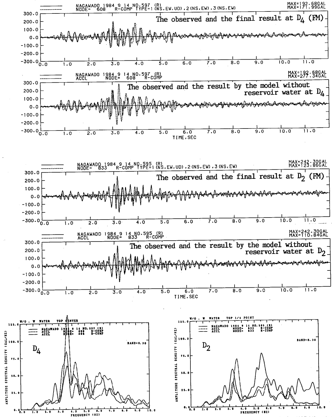
Figure 2.2.26 Comparison of the simulated results obtained by the model without reservoir water with the final result; For time histories, line type is same as Figure 2.2.22. For spectra, solid, dotted, and chained lines are for those of the observed, the final results, and the results by the model of this case.
