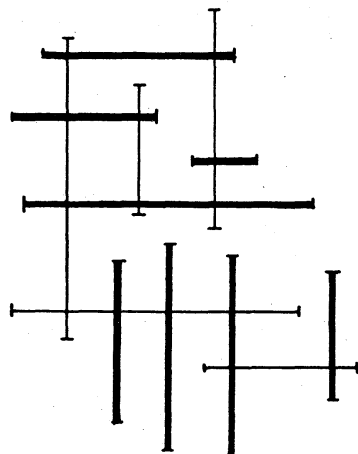
Fig.4.3. Maximum number of non-intersecting segments
